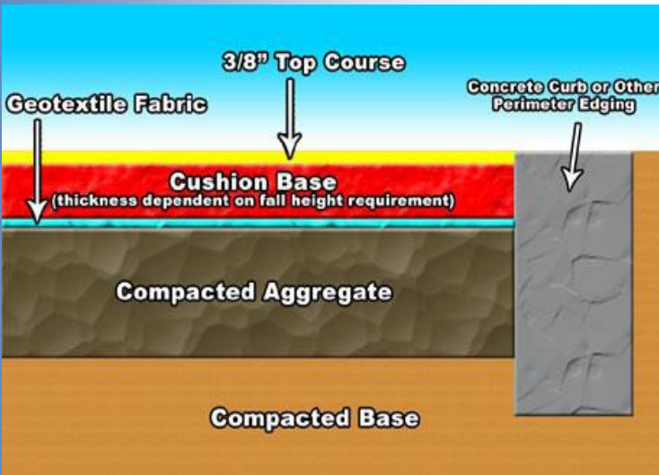
Concrete Curb or Similar Edging
