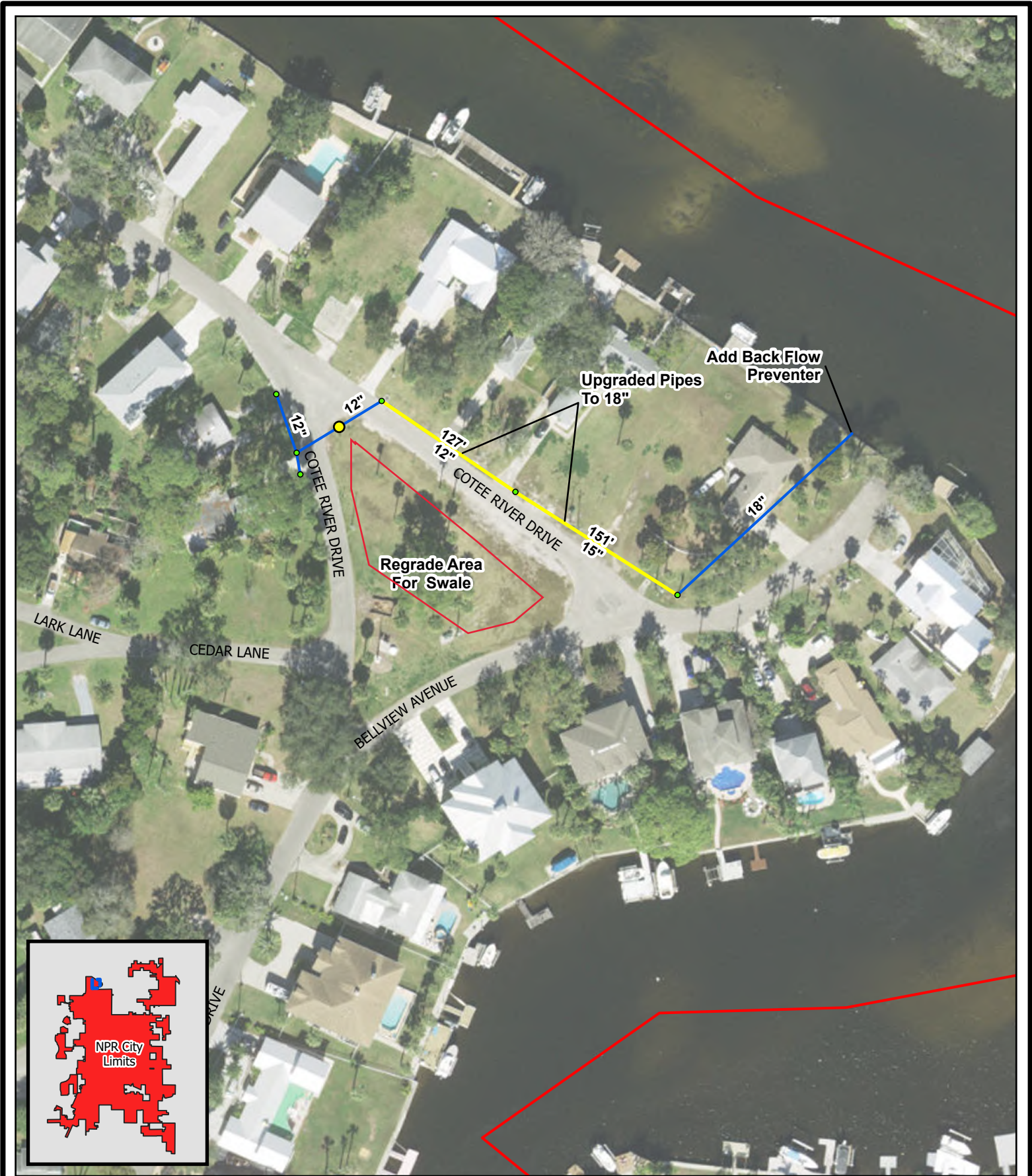
Figure 7-6. Stormwater Master Plan Proposed Projects - Cottee River Drive NPR SWMP Update New Port Richey, FL
