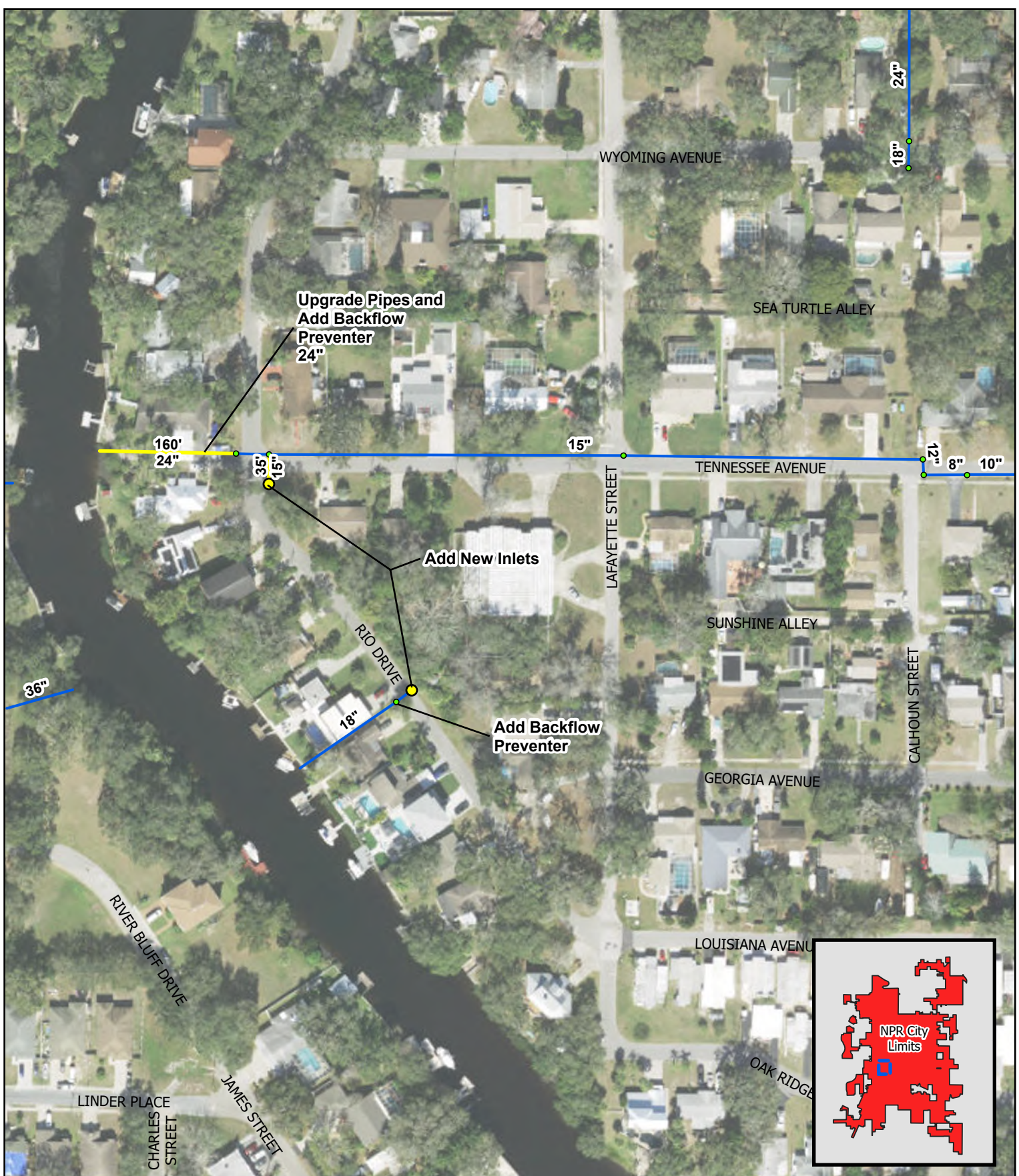
Figure 7-8. Stormwater Master Plan Proposed Projects - Rio Drive NPR SWMP Update New Port Richey, FL
