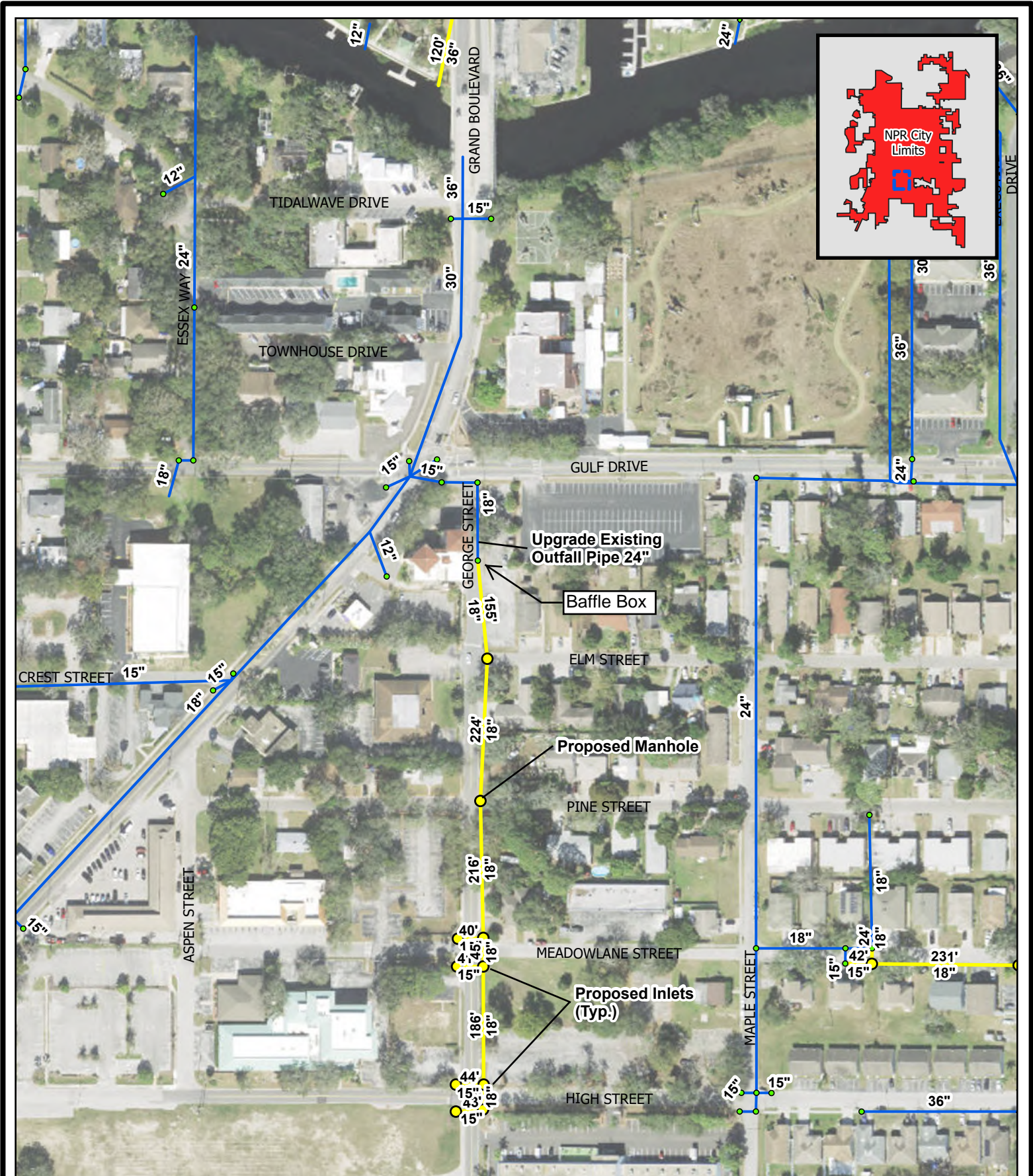
Figure 7-9. Stormwater Master Plan Proposed Projects - George Street from Elm Street to High Street
