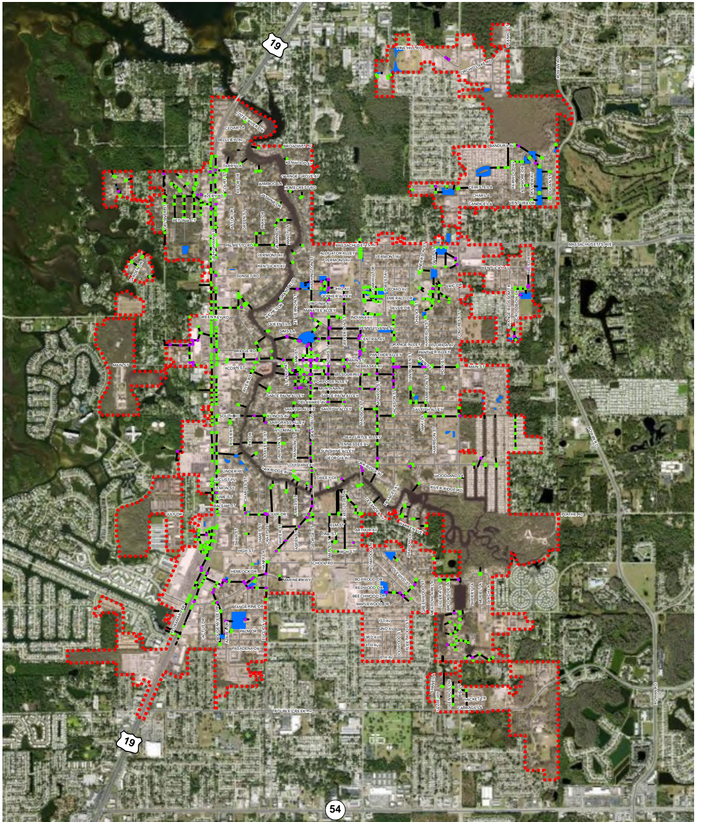
Figure 6-4 Existing Stormwater Drainage System New Port Richey Stormwater Masterplan Update New Port Richey, FL
