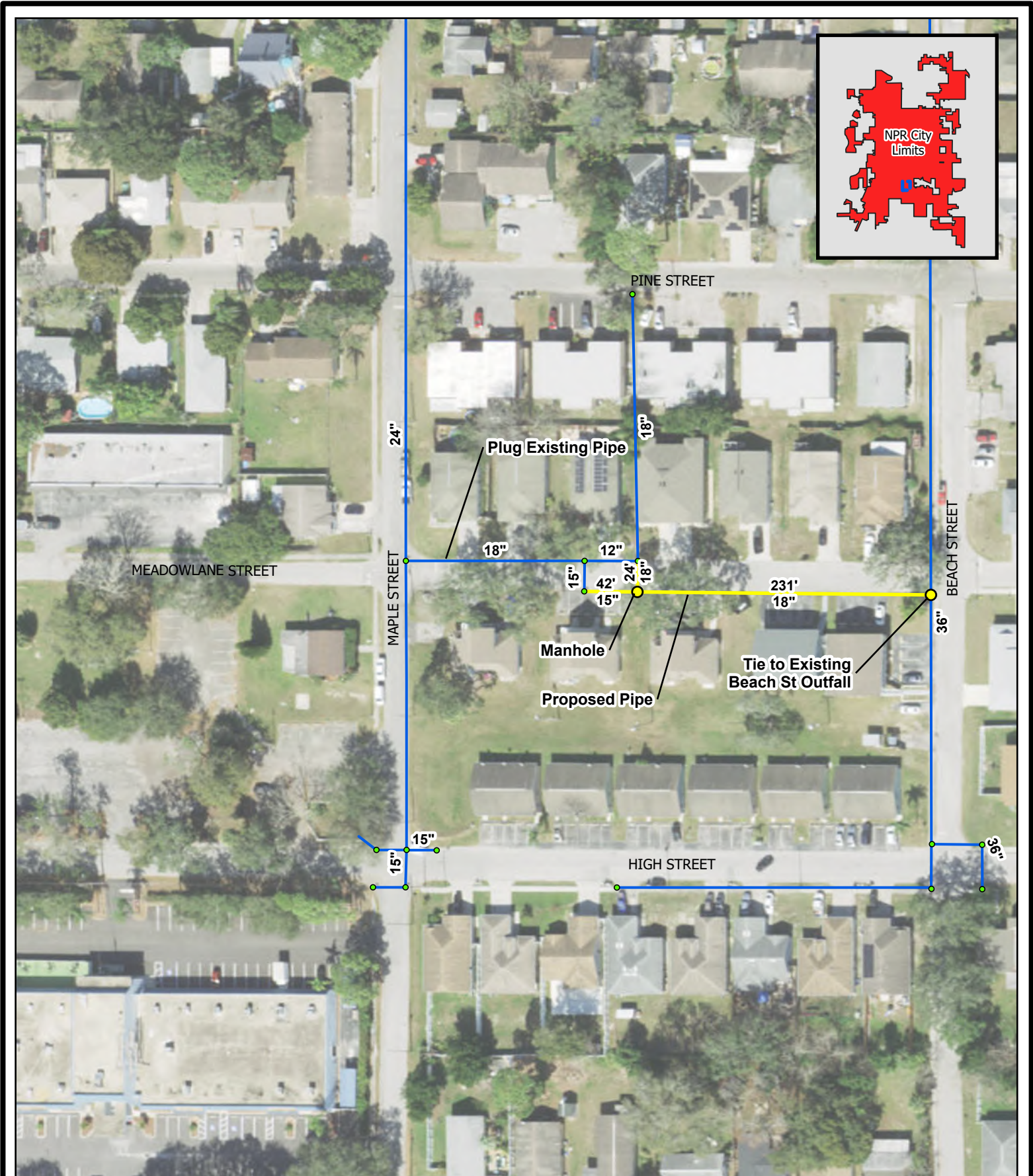
Figure 7-5. Stormwater Master Plan Proposed Projects - Maple St and Meadow Lane NPR SWMP Update New Port Richey, FL
