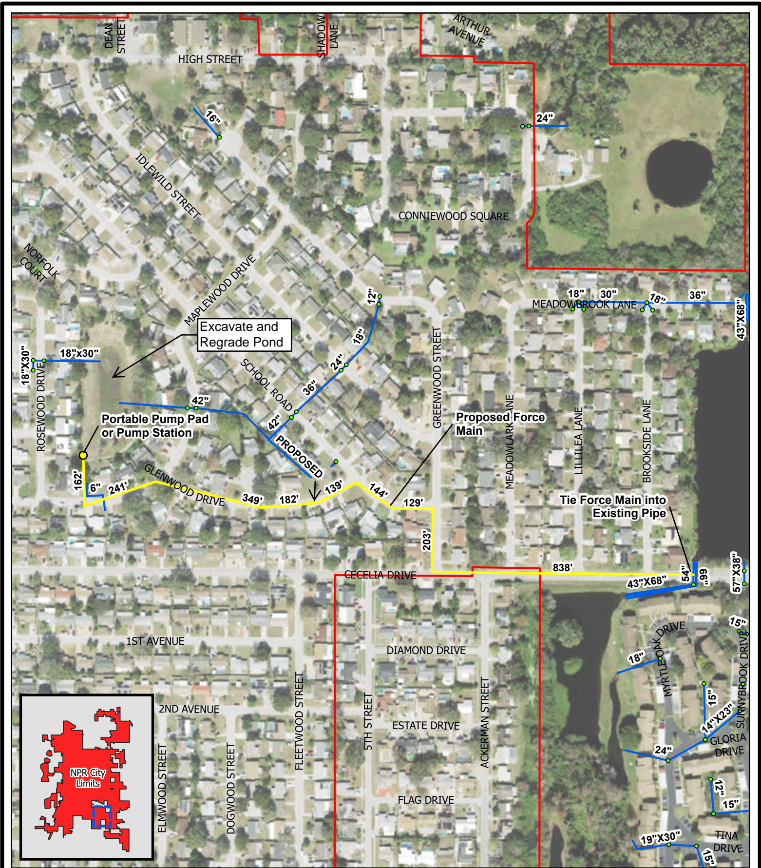
Figure 7-1. Stormwater Master Plan Proposed Projects - Tanglewood Pond Outfall Improvements NPR SWMP Update New Port Richey, FL
