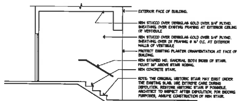
5 SECTION AT NEW MAIN EXTERIOR STAIR AB.3 SCALE: 1/4"=1'-0"
