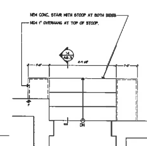
13 PLAN AT NEW EXTERIOR STAIR AB.3 SCALE: 1/2"=1'-0"
