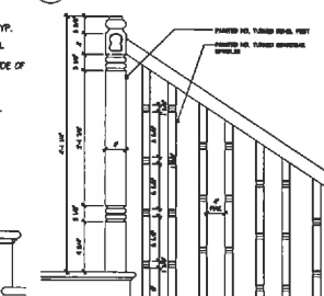
8 NEWEL POST / SPINDLE DETAIL AB 3 SCALE: 1"=1'-0"
