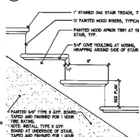
9 STAIR RISER / TREAD DETAIL A8.3 SCALE: 1"=1'-0"
