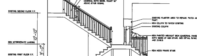
3 SECTION AT NEW MAIN LOBBY STAIR AB.3 SCALE: 1/4"=1'-0"
