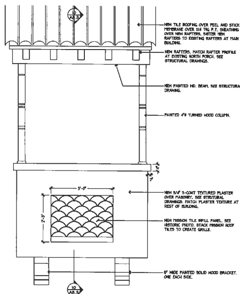
12 ELEVATION • NEW BALCONY A.B.3 SCALE: 3/4"=1'-0"
