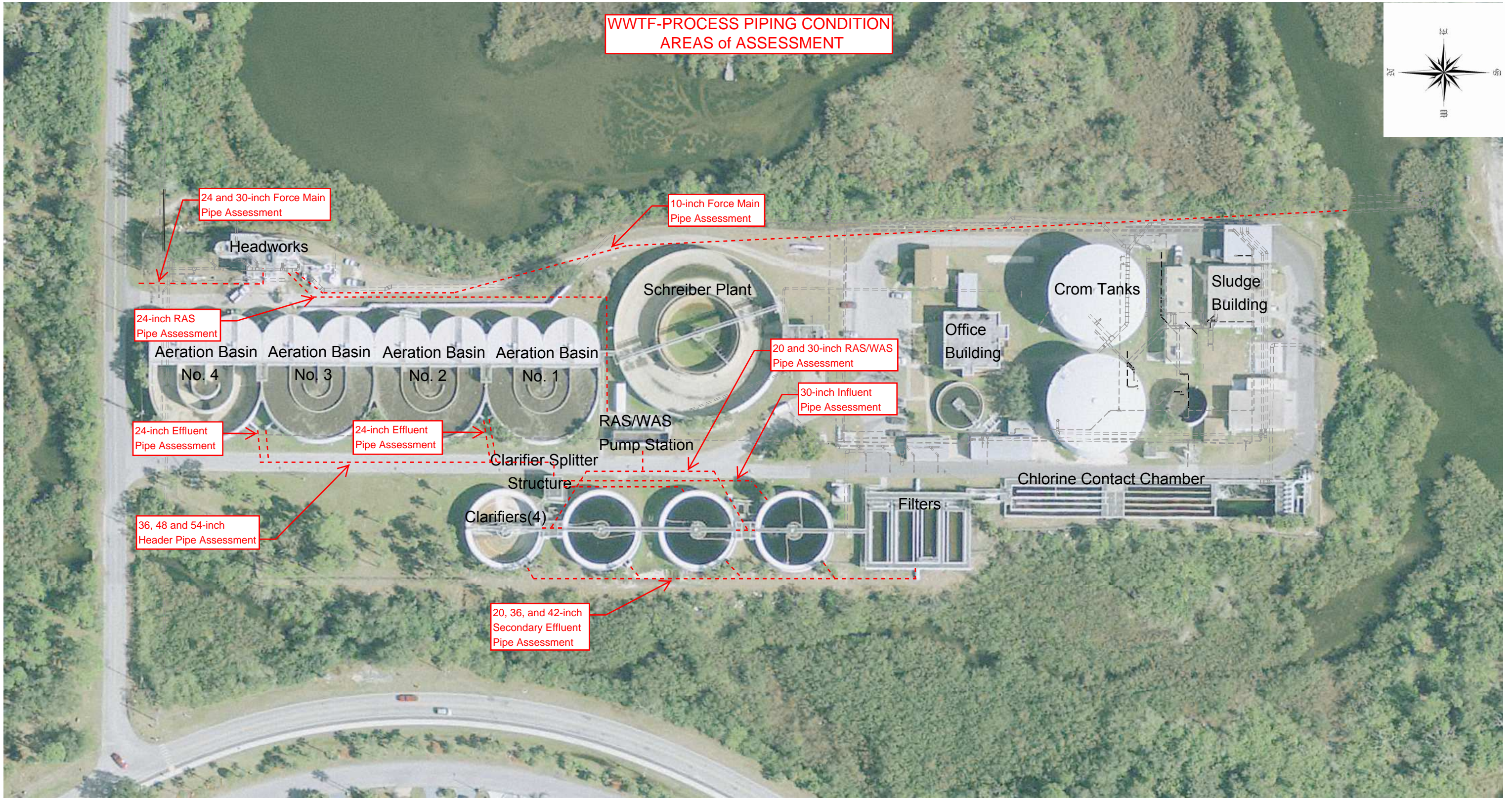
WASTEWATER TREATMENT PLANT - NORTH CITY OF NEW PORT RICHEY
